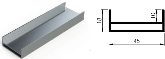
PERFIL U FIJO PA U PROFILE PA FIX PA SYSTEM
